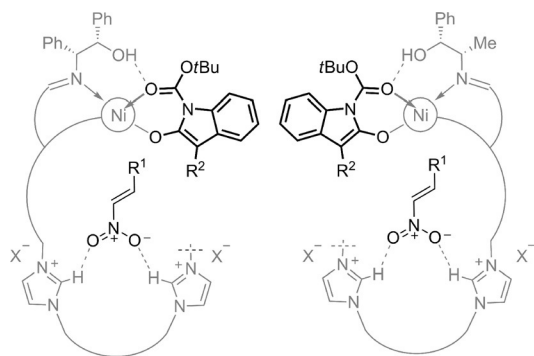
Figure 2. Simplified working model: whereas the preferred spatial orientation of the nitroolefin is mainly determined by the axially chiral bisimidazolium linker and thus similar for catalysts 1a (left) and 1b (right), the reactive orientation of the nucleophile depends on the iminoalcohol side chain (only the iminoalcohol moiety involved in a hydrogen bond with the substrate is shown for simplicity).
