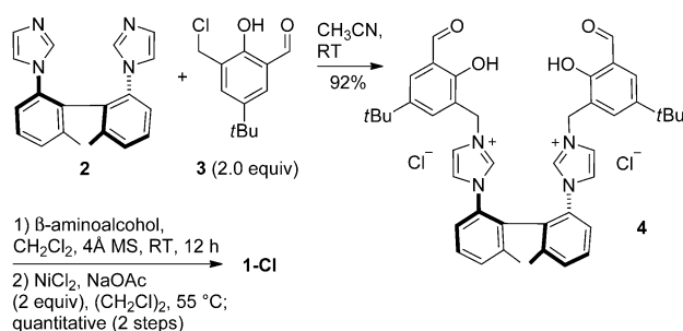
Scheme 1. Synthesis of the catalysts 1-Cl .
