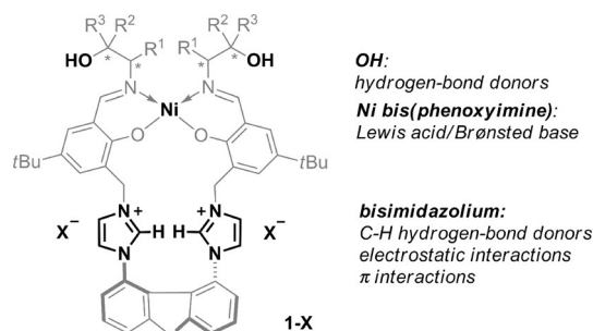
Figure 1. General design of the polyfunctional catalysts 1-X .
